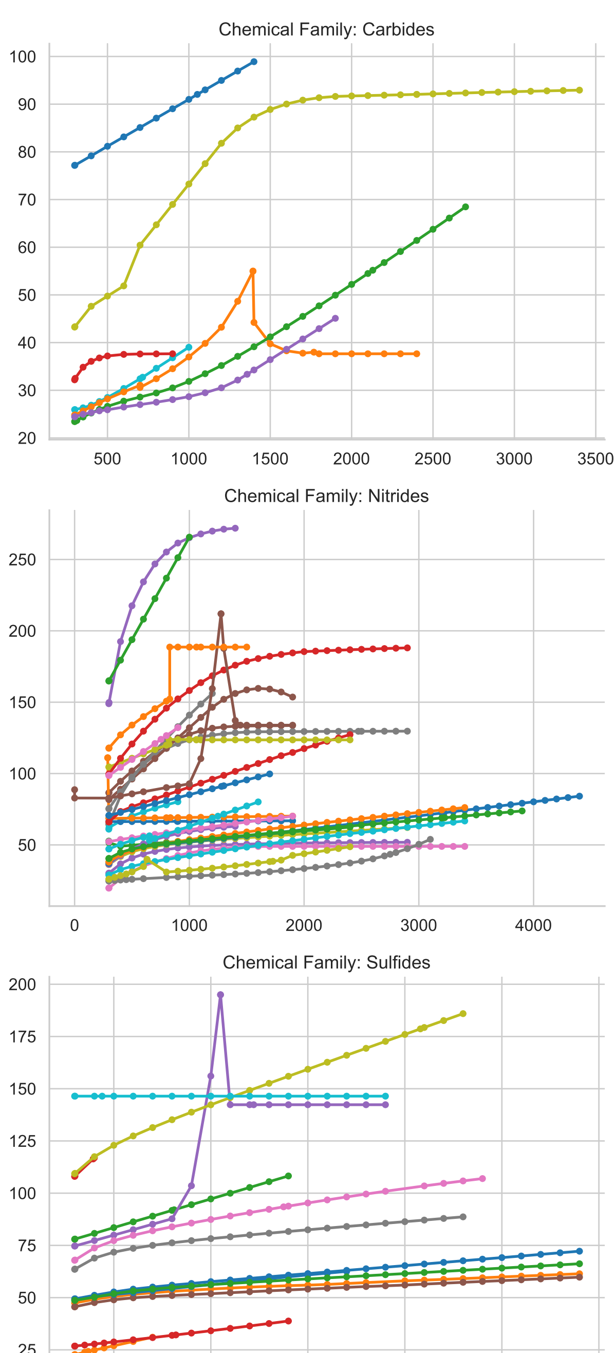
Cp vs Temperature Across Chemical Families
